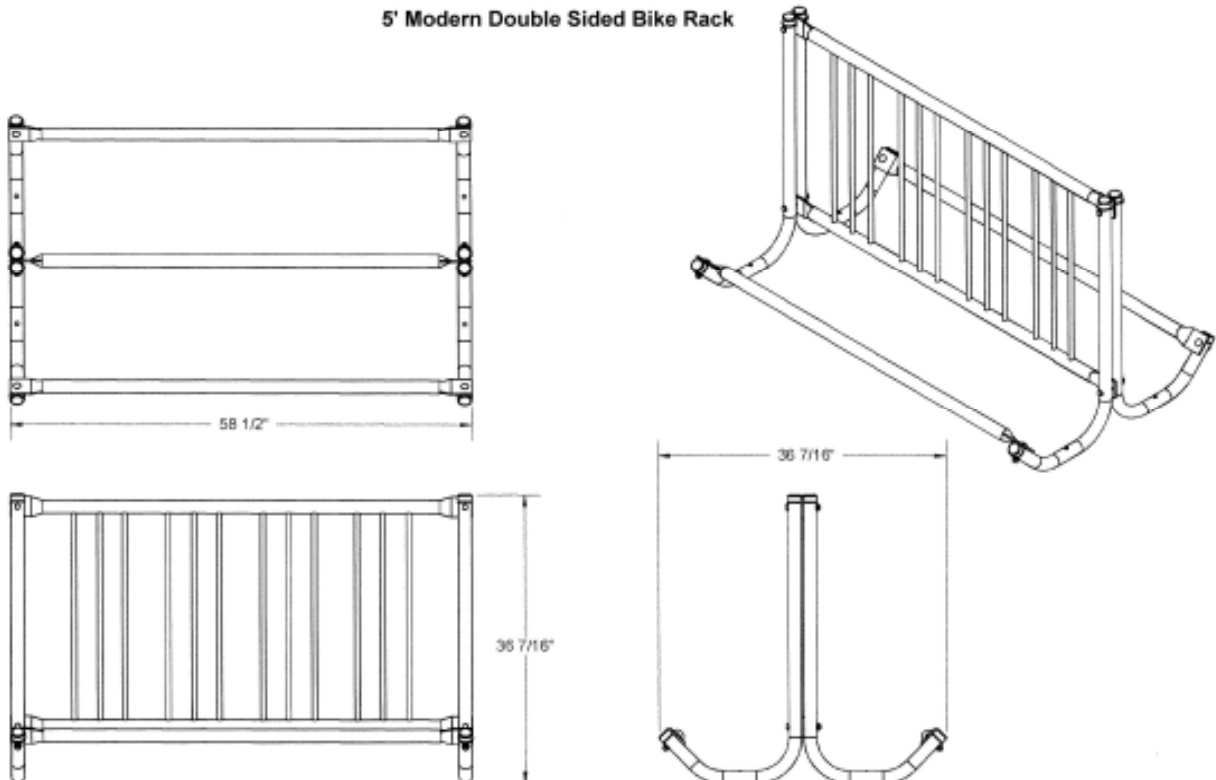
5' Modern Double Sided Bike Rack
