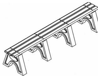
3D ISOMETRIC VIEW
