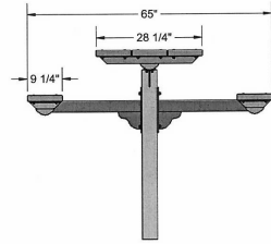
Inground Mount
