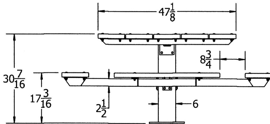
FRONT/SIDE VIEW
