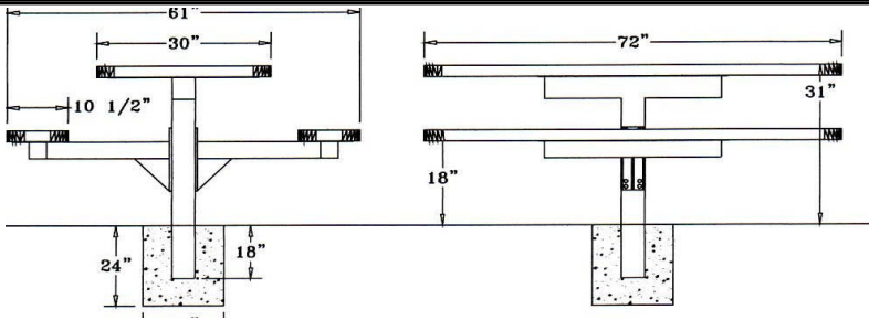
6' Perforated Style Inground Mount
