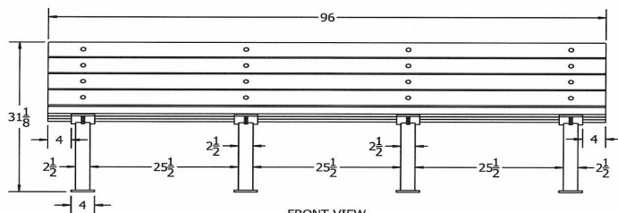
FRONT VIEW
