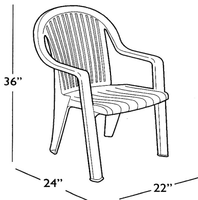
Sandstone
